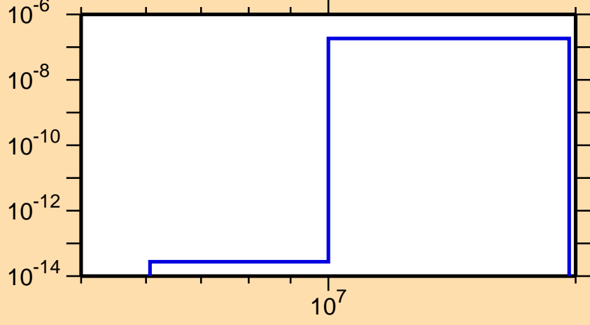
\sigma vs. E for ^{120}\text{Cs}(\text{mt117})
