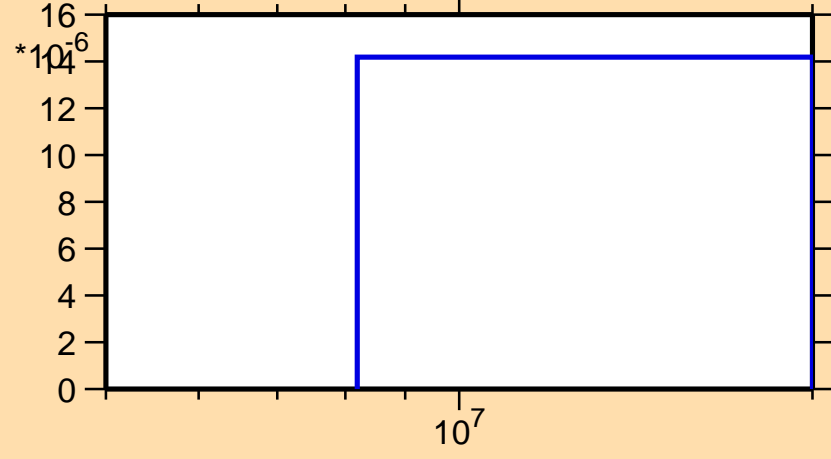
\sigma vs. E for ^{120}\text{Cs}(n,nd)
