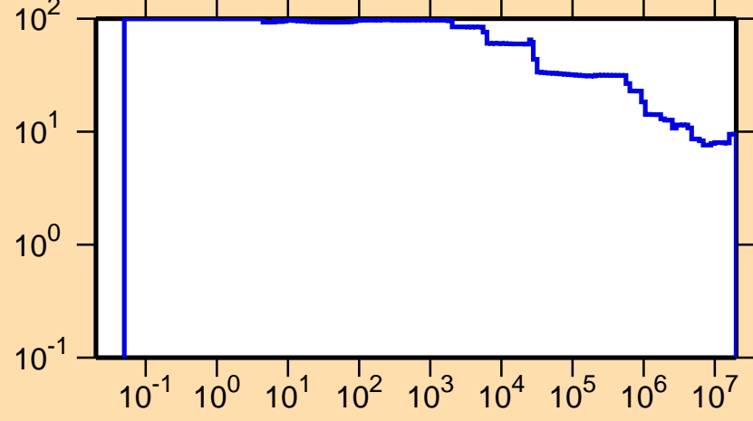
\Delta\sigma/\sigma vs. E for ^{120}\text{Cs}(n,n\text{onel.})
