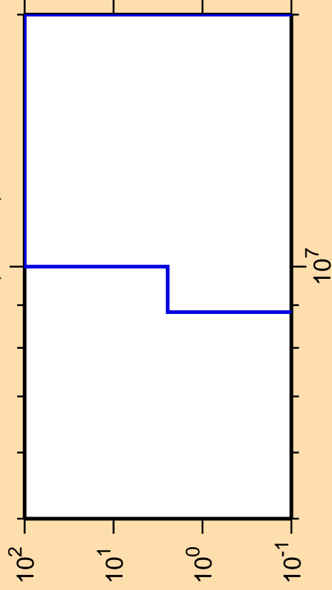
\Delta\sigma/\sigma vs. E for ^{120}\text{Cs} (mt 45)
