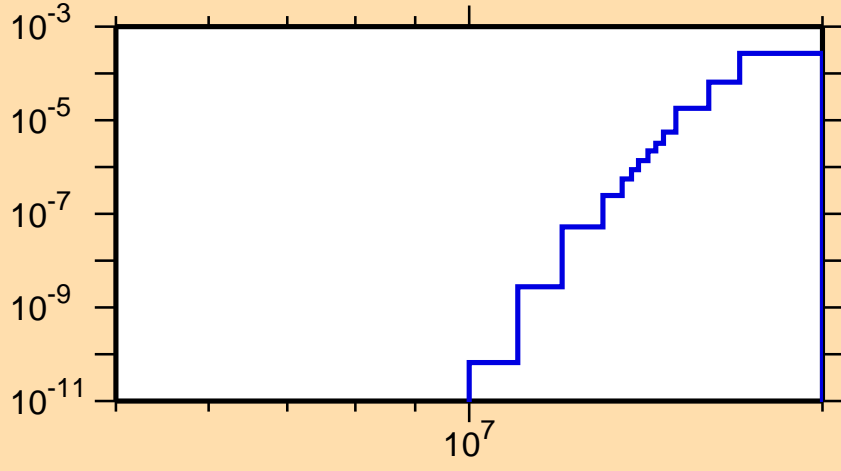
\sigma vs. E for ^{120}\text{Cs} (mt 45)
