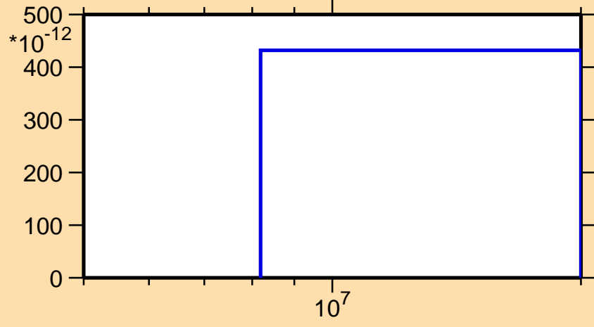
\sigma vs. E for ^{120}\text{Cs}(\text{mt } 34)
