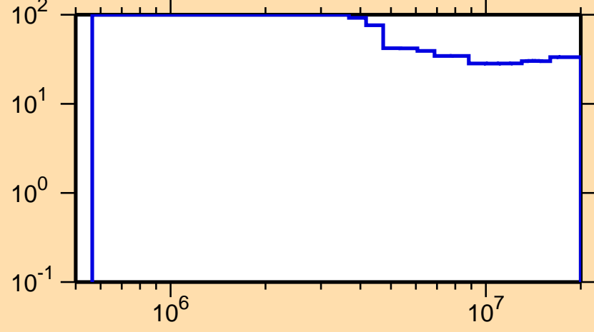
\Delta\sigma/\sigma vs. E for ^{121}\text{Cs}(n,ncont.)
