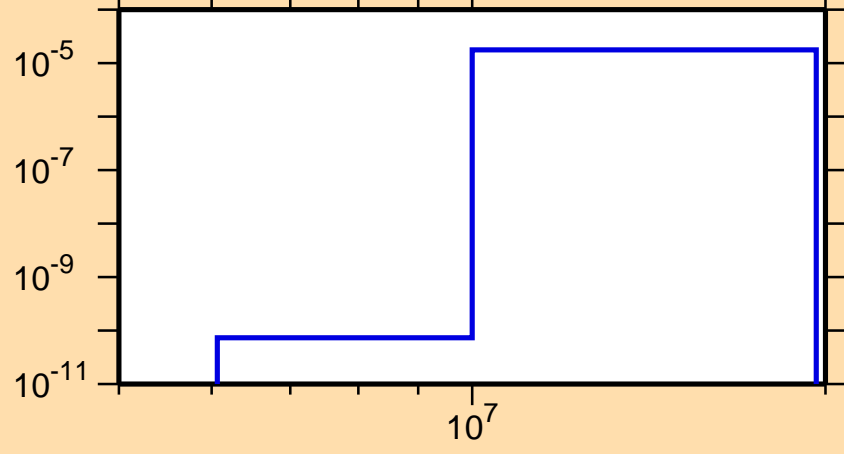
\sigma vs. E for ^{121}\text{Cs}(n,\text{He3})
