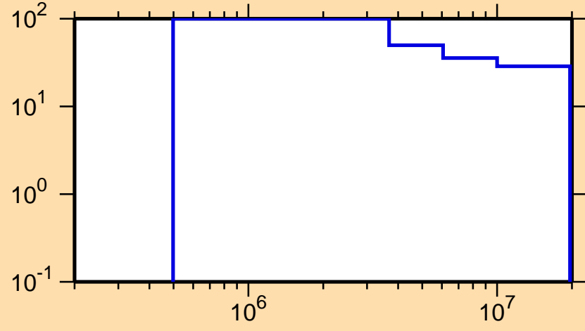
\Delta\sigma/\sigma vs. E for ^{121}\text{Cs}(n,n\text{cont.})
