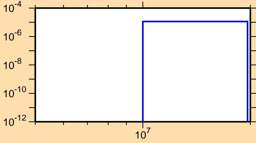
\sigma vs. E for ^{121}\text{Cs} (mt 45)
