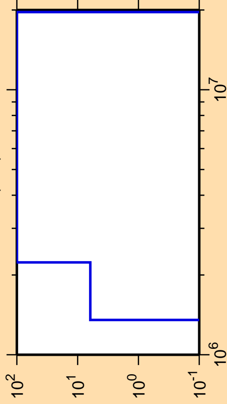
\Delta\sigma/\sigma vs. E for ^{121}\text{Cs}(n,d)
