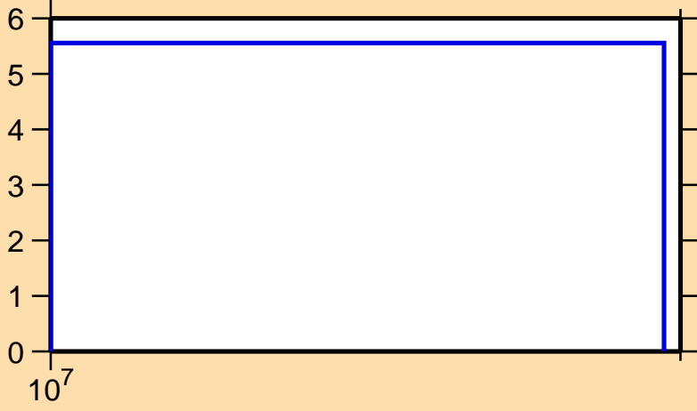
\Delta\sigma/\sigma vs. E for ^{121}\text{Cs}(n,\text{el.})
