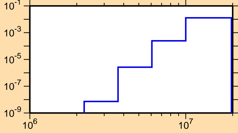
\sigma vs. E for ^{121}\text{Cs}(n,d)
