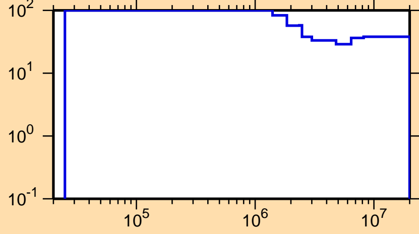
\Delta\sigma/\sigma vs. E for ^{121}\text{Cs}(n,n_1)
