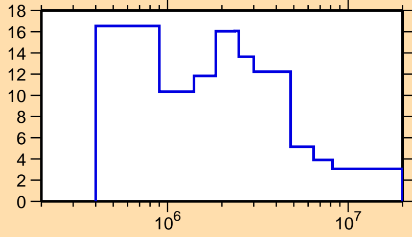
\Delta\sigma/\sigma vs. E for ^{121}\text{Cs}(n,tot.)
