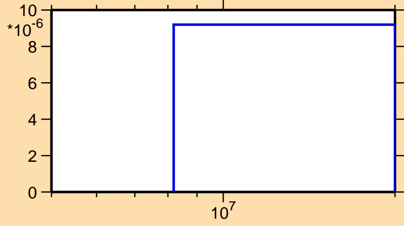
\sigma vs. E for ^{121}\text{Cs}(\text{mt } 45)
