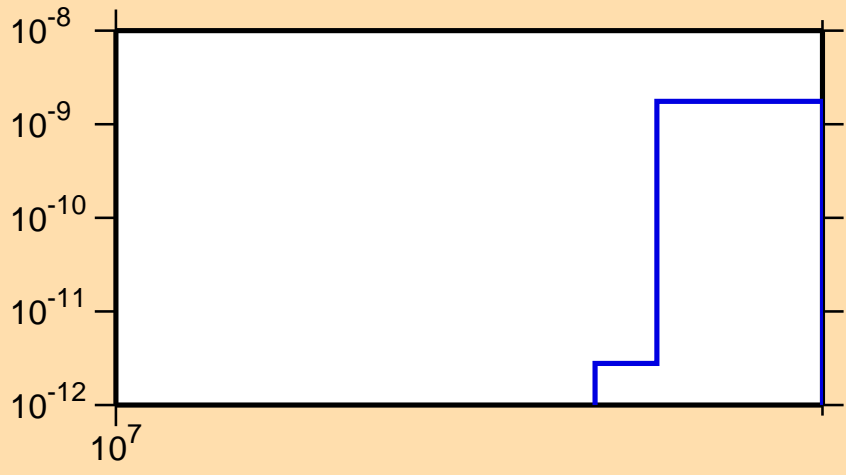
\sigma vs. E for ^{121}\text{Cs}(n,pt)
