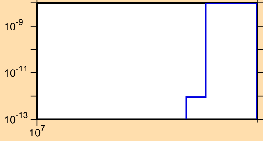
\sigma vs. E for ^{121}\text{Cs}(n,nt)
