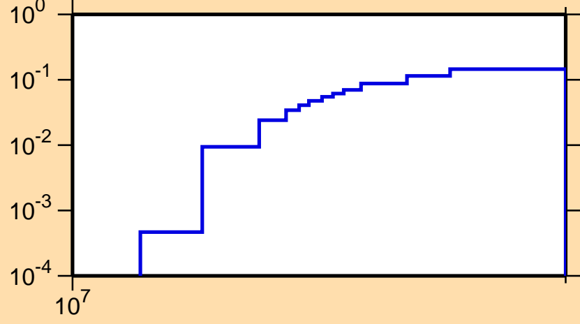
\sigma vs. E for ^{121}\text{Cs}(n,2n)
