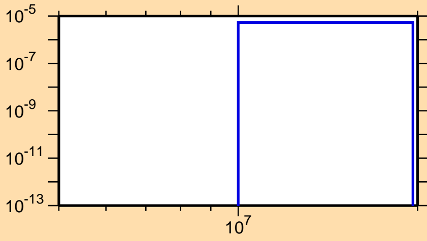
\sigma vs. E for ^{121}\text{Cs}(\text{mt } 45)
