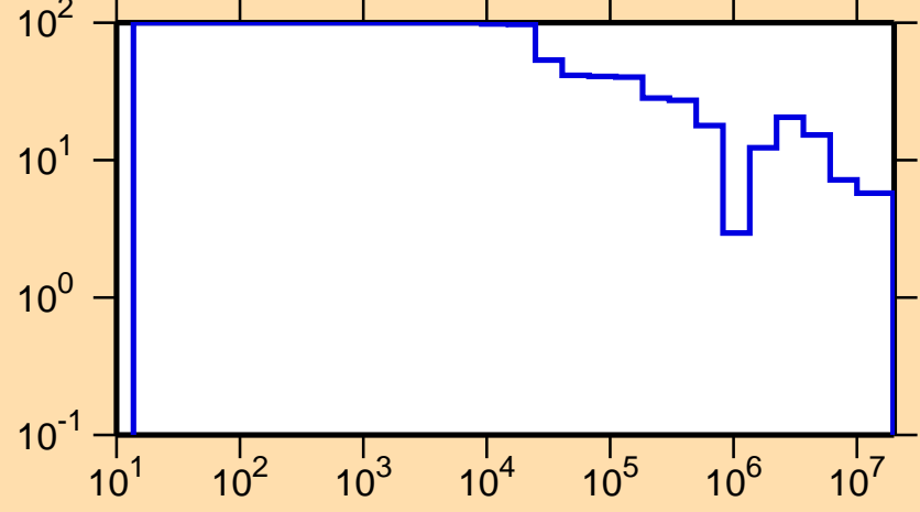
\Delta\sigma/\sigma vs. E for ^{121}\text{Cs}(n,\text{el.})
