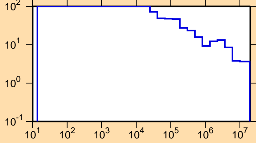
\Delta\sigma/\sigma vs. E for ^{121}\text{Cs}(n,\text{tot.})
