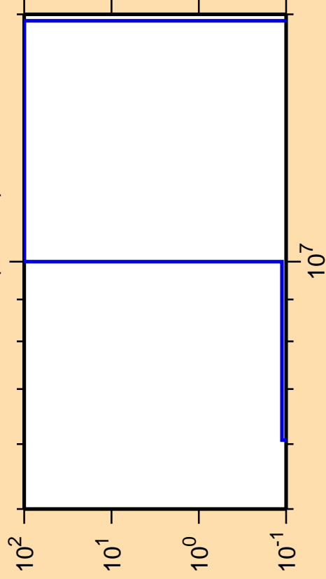
\Delta\sigma/\sigma vs. E for ^{121}\text{Cs}(\text{mt } 45)
