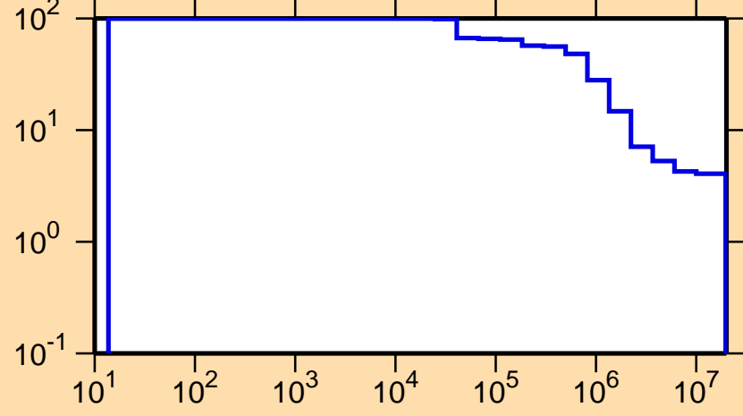
\Delta\sigma/\sigma vs. E for ^{121}\text{Cs}(n,\text{nonel.})
