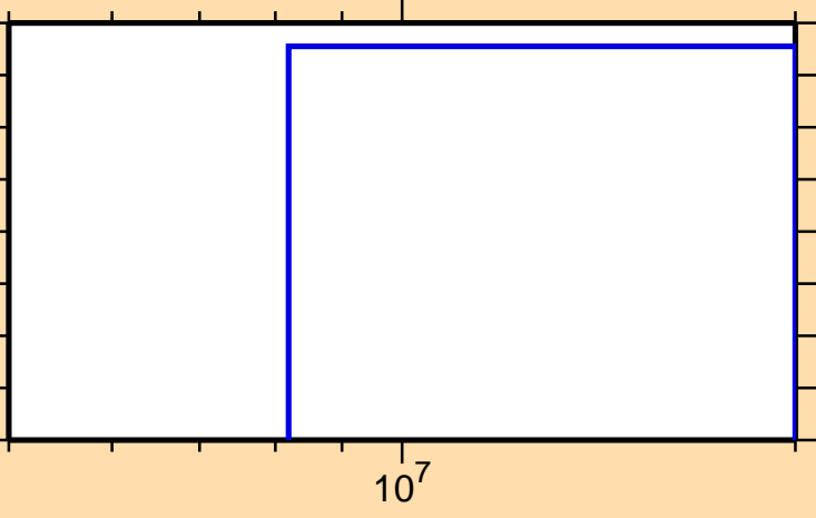
\sigma vs. E for ^{121}\text{Cs}(n,2n)
