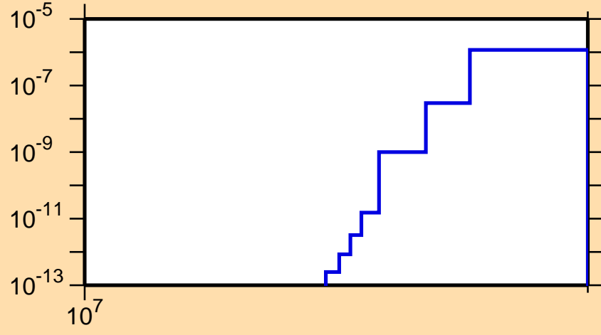
\sigma vs. E for ^{122}\text{Cs}(n,pt)
