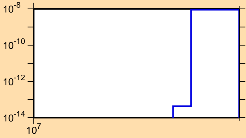
\sigma vs. E for ^{122}\text{Cs}(n,nt)
