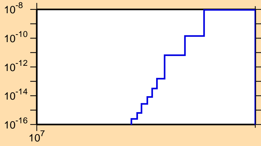
\sigma vs. E for ^{122}\text{Cs} (mt 34)
