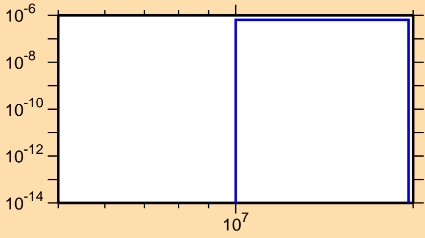
\sigma vs. E for ^{122}\text{Cs}(\text{mt } 45)
