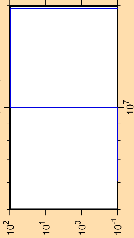
\Delta\sigma/\sigma vs. E for ^{122}\text{Cs}(\text{mt } 45)
