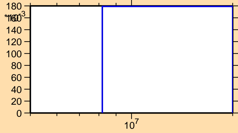
\sigma vs. E for ^{122}\text{Cs}(n,2n)
