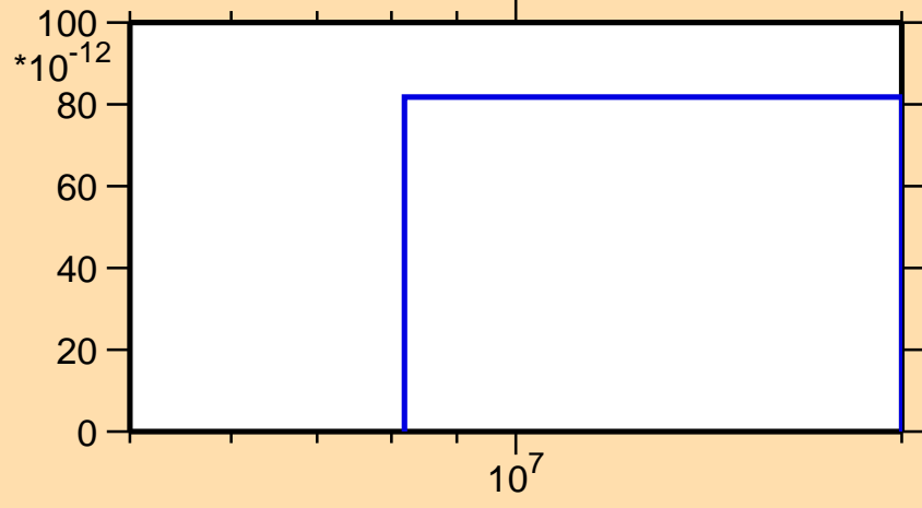
\sigma vs. E for ^{122}\text{Cs}(\text{mt } 34)
