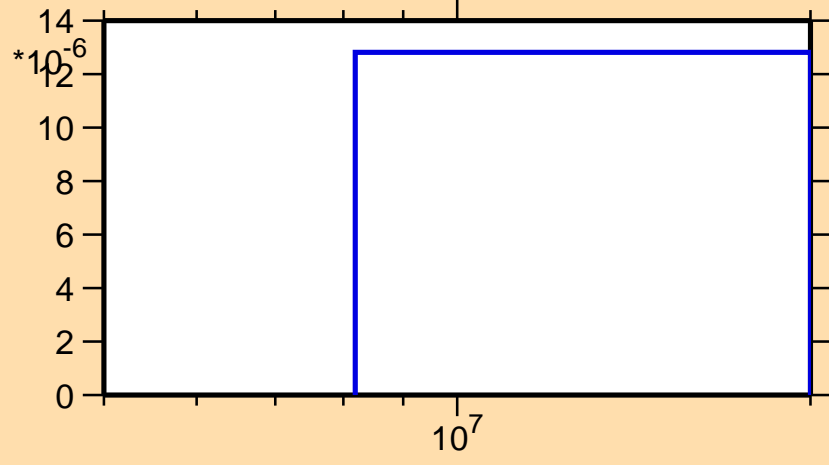
\sigma vs. E for ^{122}\text{Cs}(n,\text{nd})
