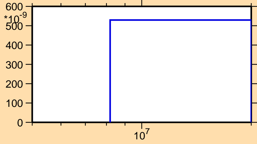
\sigma vs. E for ^{122}\text{Cs} (mt 45)
