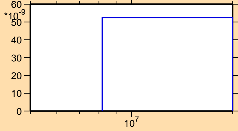
\sigma vs. E for ^{122}\text{Cs}(n,\text{pd})
