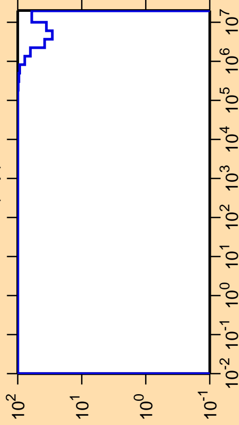
\Delta\sigma/\sigma vs. E for ^{122}\text{Cs}(n,p)
