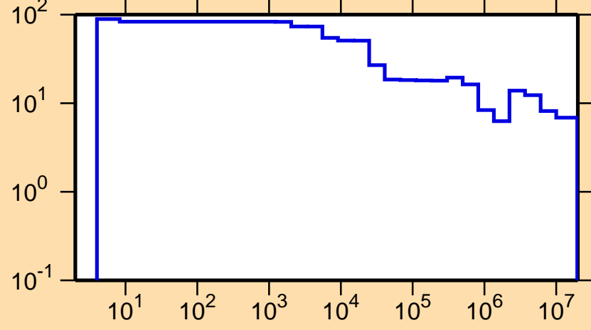
\Delta\sigma/\sigma vs. E for ^{122}\text{Cs}(n,\text{el.})
