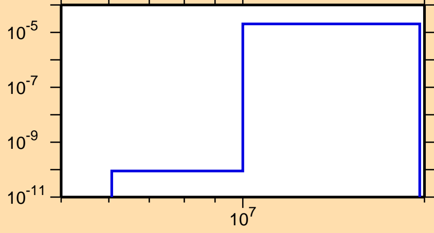
\sigma vs. E for ^{122}\text{Cs}(n,\text{He3})
