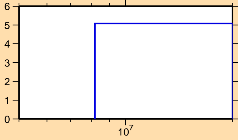
\Delta\sigma/\sigma vs. E for ^{122}\text{Cs}(n,\text{nonel.})
