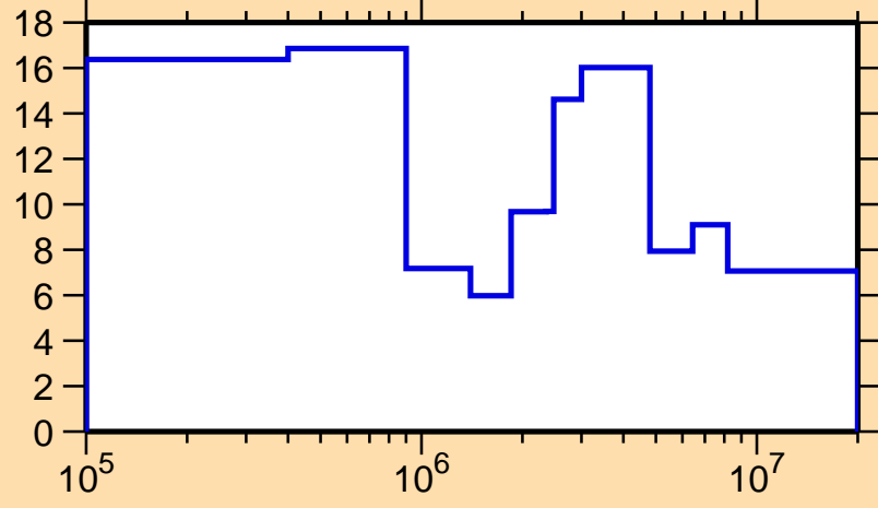
\Delta\sigma/\sigma vs. E for ^{122}\text{Cs}(n, el.)
