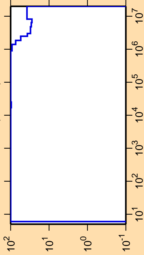
\Delta\sigma/\sigma vs. E for ^{122}\text{Cs}(n,\text{inel.})
