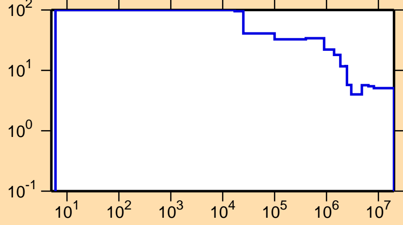
\Delta\sigma/\sigma vs. E for ^{122}\text{Cs}(n,\text{nonel.})
