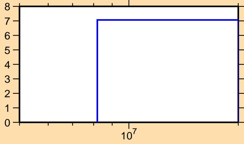
\Delta\sigma/\sigma vs. E for ^{122}\text{Cs}(n,\text{el.})
