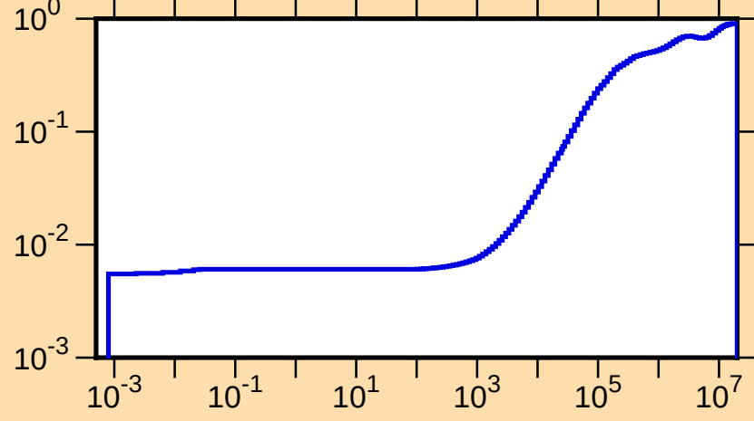
\mu vs. E for ^{123}\text{Cs}(\text{mt251})
