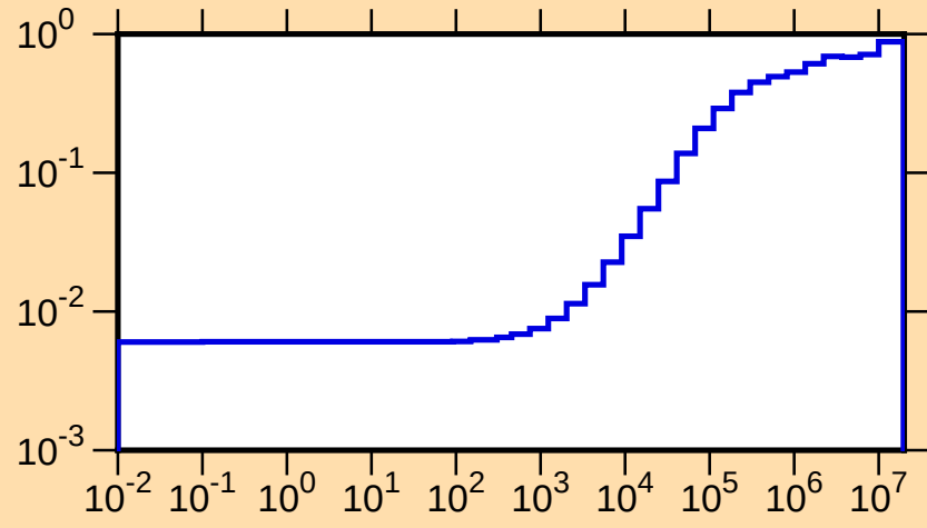
\mu vs. E for ^{123}\text{Cs}(\text{mt251})
