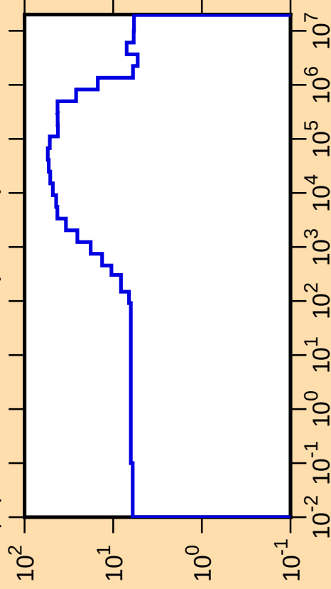
\Delta\mu/\mu vs. E for ^{123}\text{Cs}(\text{mt251})
