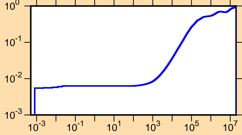
\mu vs. E for ^{124}\text{Cs}(\text{mt251})
