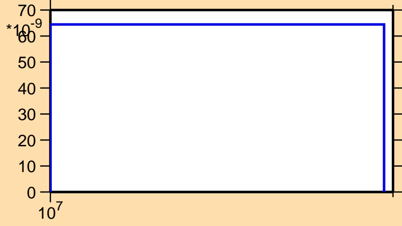
\sigma vs. E for ^{124}\text{Cs}(n,2n\alpha)
