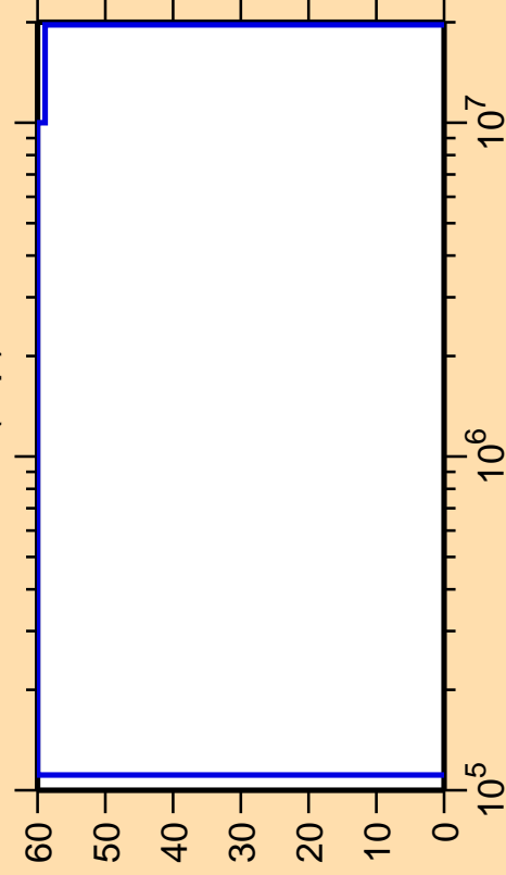
\Delta\sigma/\sigma vs. E for ^{124}\text{Cs}(n,p)
