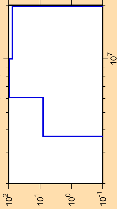
\Delta\sigma/\sigma vs. E for ^{124}\text{Cs}(n,n\alpha)
