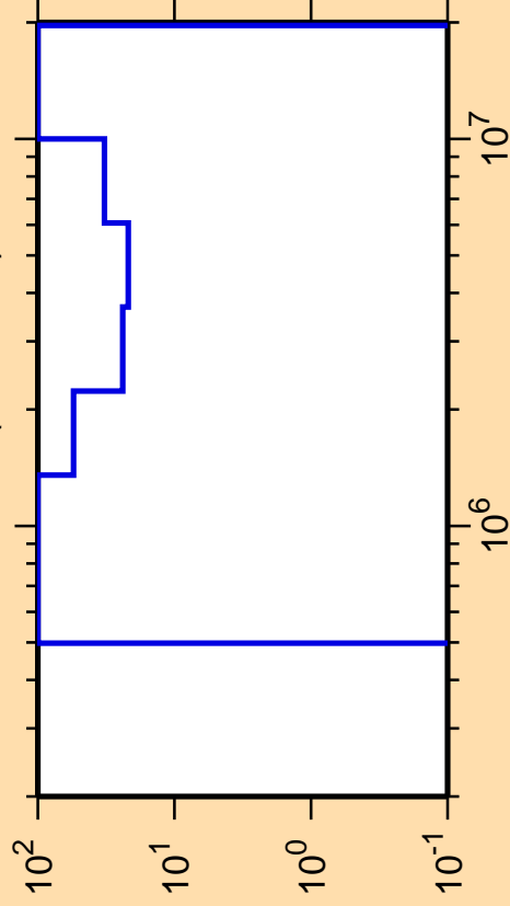
\Delta\sigma/\sigma vs. E for ^{124}\text{Cs}(n,n\text{cont.})
