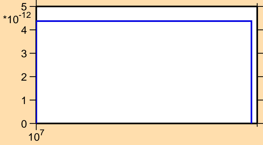
\sigma vs. E for ^{124}\text{Cs} (mt 34)
