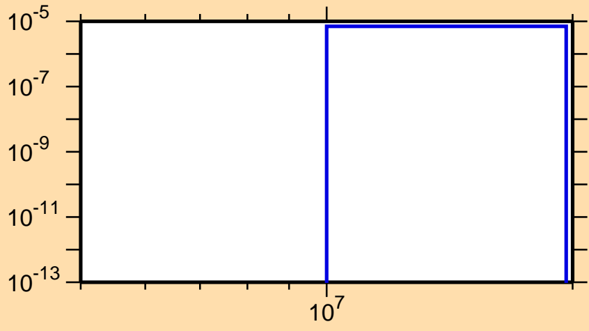
\sigma vs. E for ^{124}\text{Cs}(n,nd)
