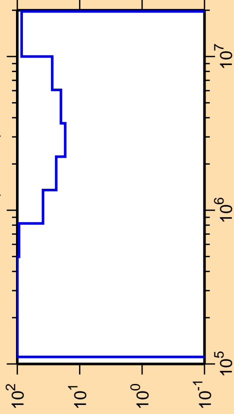
\Delta\sigma/\sigma vs. E for ^{124}\text{Cs}(n,\text{inel.})
