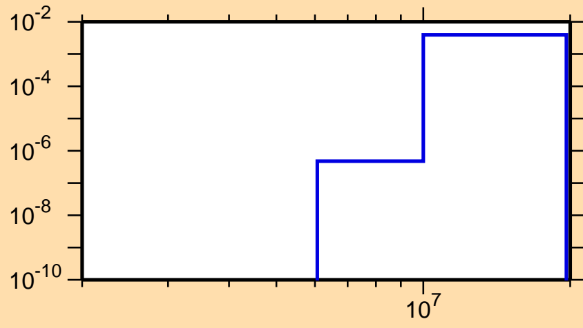
\sigma vs. E for ^{124}\text{Cs}(n,n\alpha)
