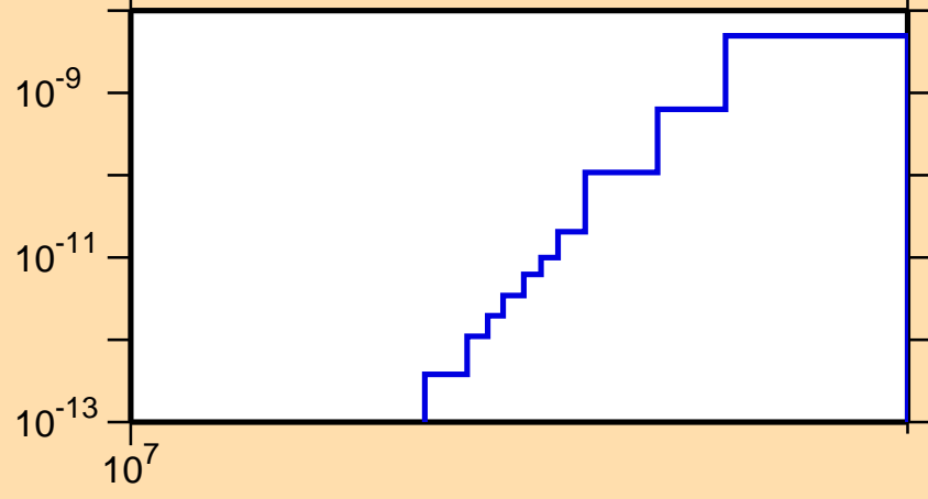
\sigma vs. E for ^{124}\text{Cs}(\text{mt117})
