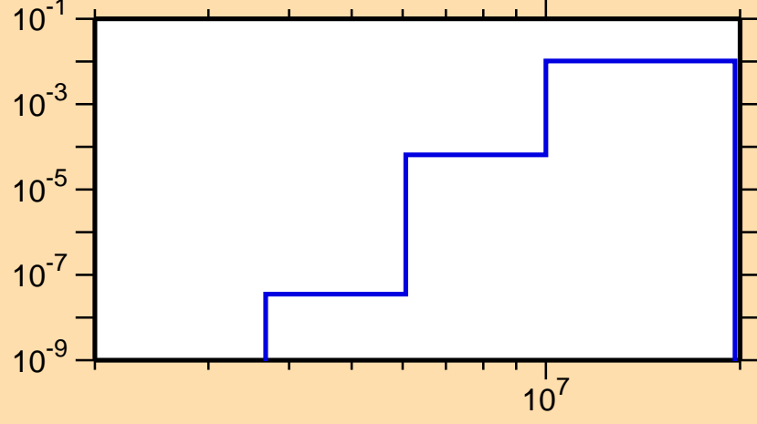
\sigma vs. E for ^{124}\text{Cs}(n,d)
