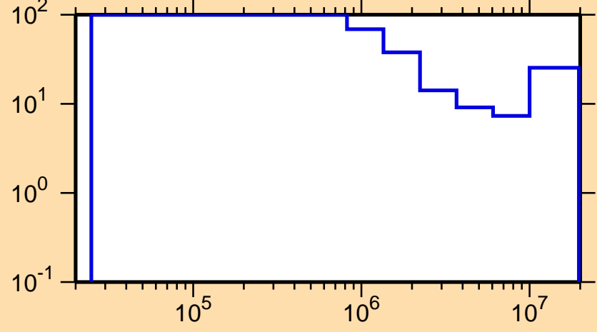
\Delta\sigma/\sigma vs. E for ^{124}\text{Cs}(n,n\text{cont.})
