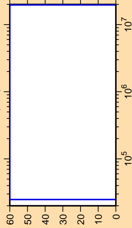
\Delta\sigma/\sigma vs. E for ^{124}\text{Cs}(n,\alpha)
