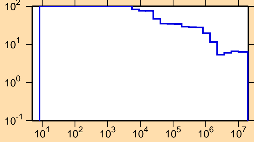
\Delta\sigma/\sigma vs. E for ^{124}\text{Cs}(n,\text{nonel.})
