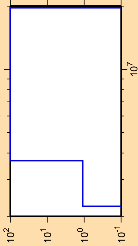
\Delta\sigma/\sigma vs. E for ^{124}\text{Cs}(n,d)
