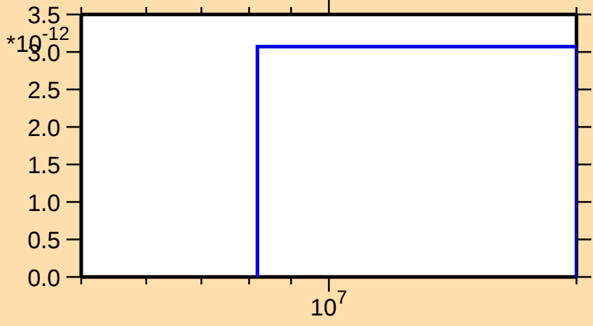
\sigma vs. E for ^{126}\text{Cs}(n,\text{pt})
