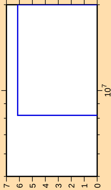
\Delta\sigma/\sigma vs. E for ^{126}\text{Cs}(\text{mt } 45)
