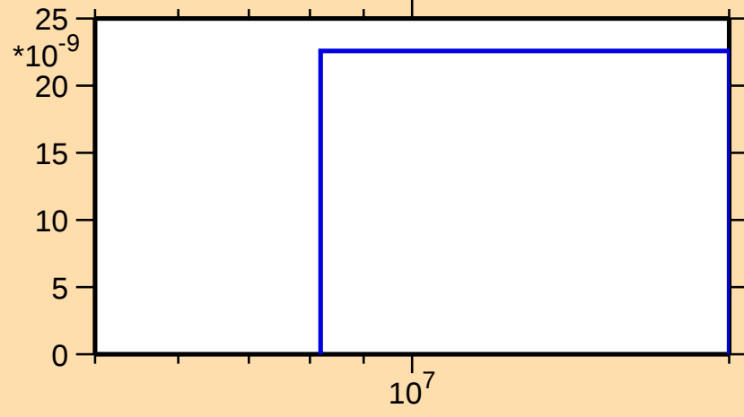
\sigma vs. E for ^{126}\text{Cs}(n,2n\alpha)
