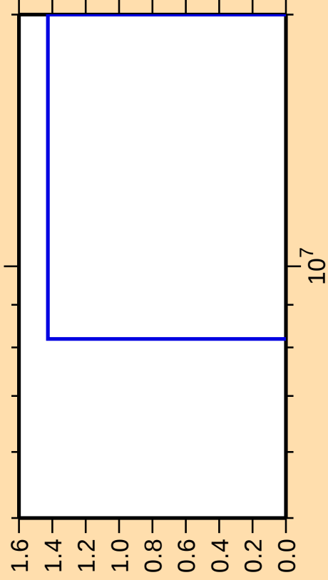
\Delta\sigma/\sigma vs. E for ^{126}\text{Cs}(\text{mt } 34)
