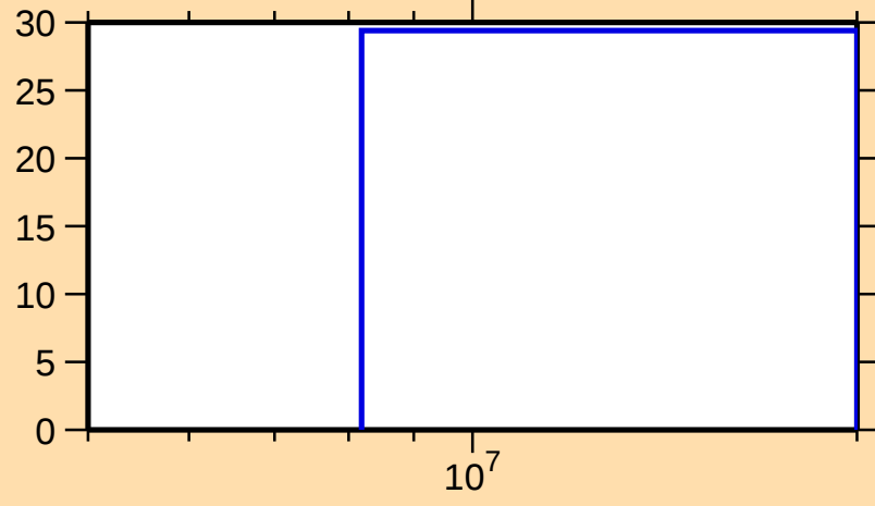
\Delta\sigma/\sigma vs. E for ^{126}\text{Cs}(n,\text{inel.})
