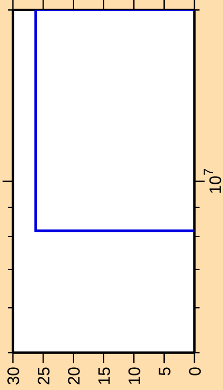
\Delta\sigma/\sigma vs. E for ^{126}\text{Cs}(n,2n)
