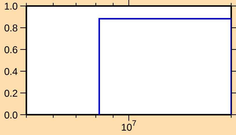
\sigma vs. E for ^{126}\text{Cs}(n,2n)
