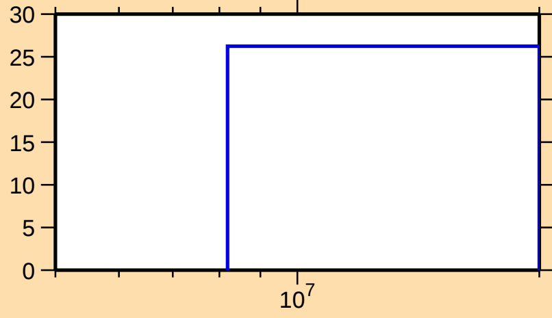
\Delta\sigma/\sigma vs. E for ^{126}\text{Cs}(n,2n)
