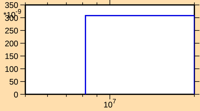
\sigma vs. E for ^{126}\text{Cs}(n,\text{He}3)
