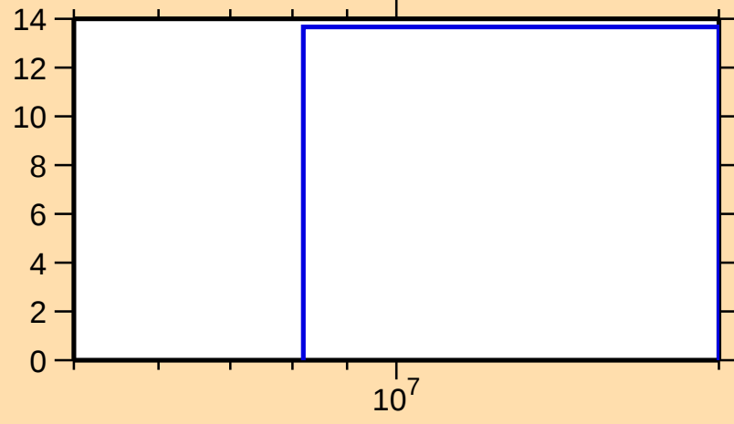
\Delta\sigma/\sigma vs. E for ^{126}\text{Cs}(n,\text{nonel.})
