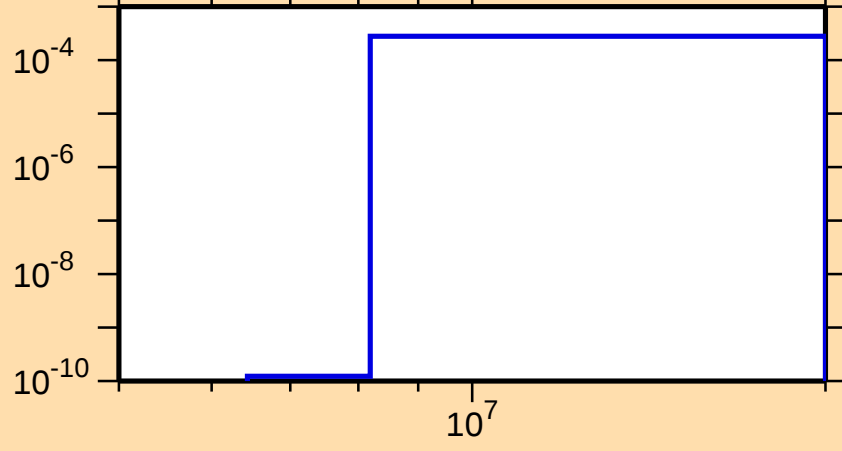
\sigma vs. E for ^{126}\text{Cs}(n,t)
