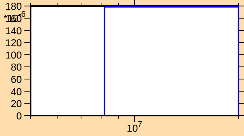
\sigma vs. E for ^{126}\text{Cs}(n,2np)
