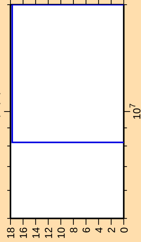
\Delta\sigma/\sigma vs. E for ^{126}\text{Cs}(n,\text{pt})
