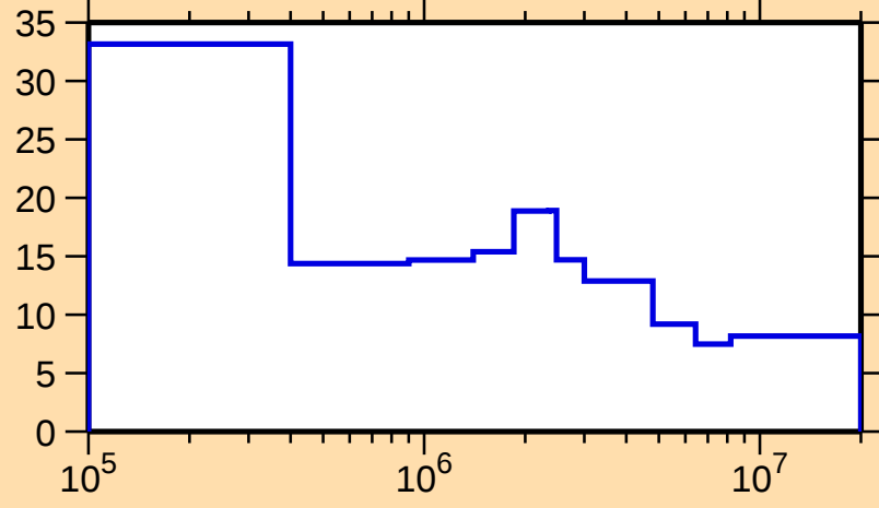
\Delta\sigma/\sigma vs. E for ^{126}\text{Cs}(n,\text{tot.})
