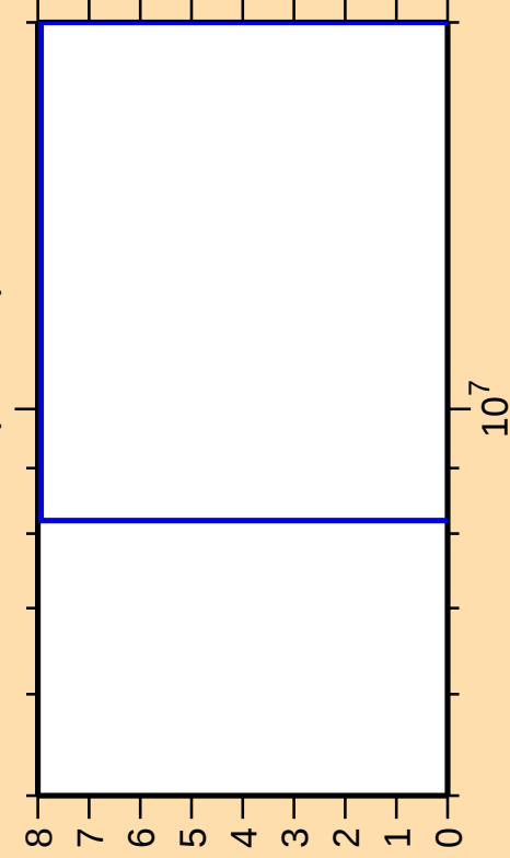
\Delta\sigma/\sigma vs. E for ^{126}\text{Cs}(\text{mt117})
