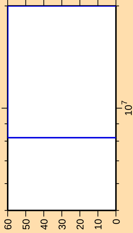
\Delta\sigma/\sigma vs. E for ^{126}\text{Cs}(n,p)
