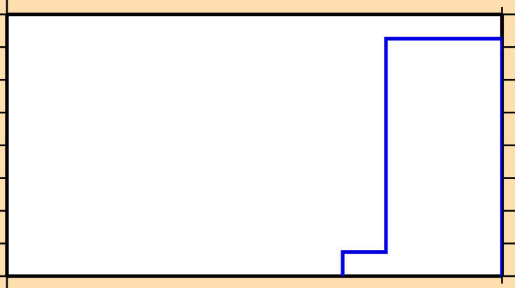
\sigma vs. E for ^{127}\text{Cs}(\text{mt117})
