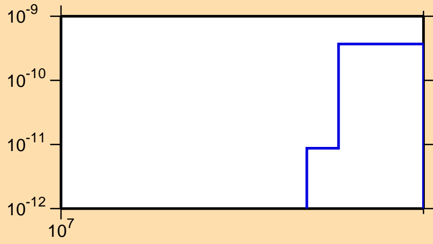
\sigma vs. E for ^{127}\text{Cs}(n,\text{pd})
