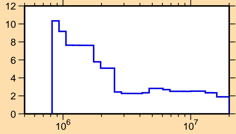
\Delta\sigma/\sigma vs. E for ^{128}\text{Cs}(n,n\text{onel.})
