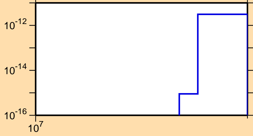
\sigma vs. E for ^{128}\text{Cs} (mt 34)
