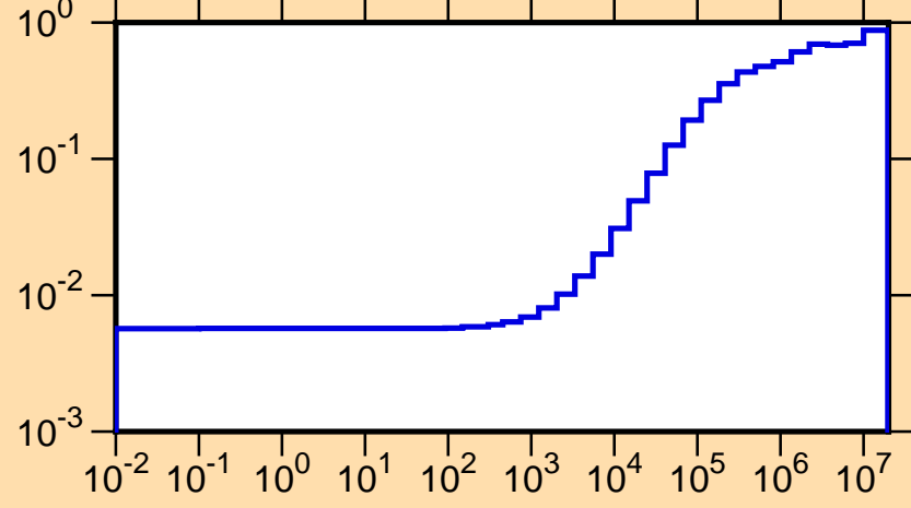
\mu vs. E for ^{128}\text{Cs}(\text{mt251})
