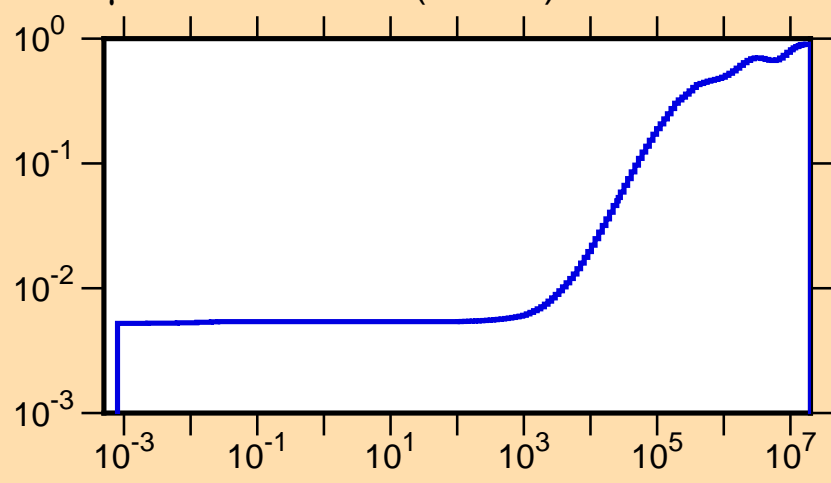
\mu vs. E for ^{129}\text{Cs}(\text{mt251})
