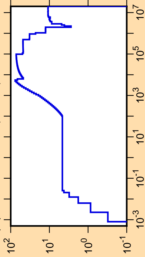
\Delta\mu/\mu vs. E for ^{129}\text{Cs}(\text{mt251})
