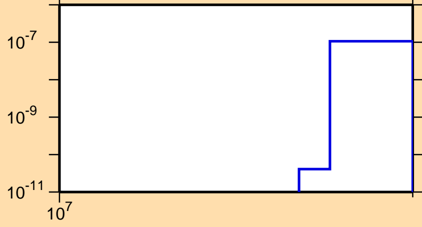
\sigma vs. E for ^{129}\text{Cs}(n,nt)
