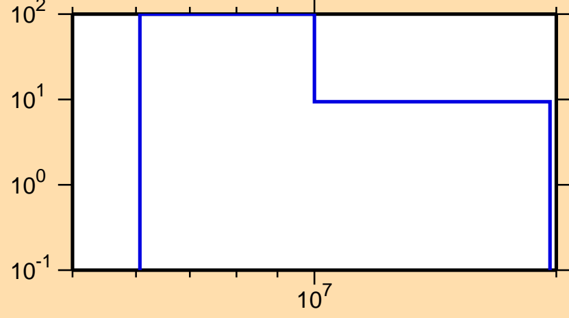
\Delta\sigma/\sigma vs. E for ^{129}\text{Cs}(n,2n)
