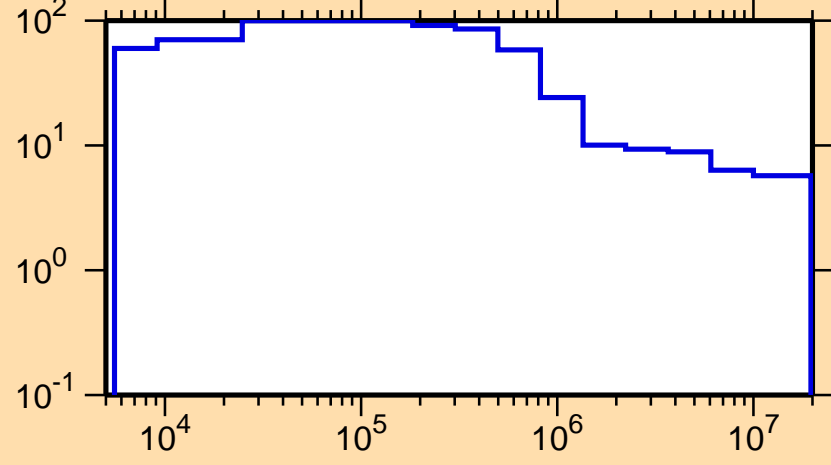
\Delta\sigma/\sigma vs. E for ^{129}\text{Cs}(n,\text{nonel.})
