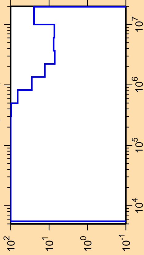
\Delta\sigma/\sigma vs. E for ^{129}\text{Cs}(n,\text{inel.})
