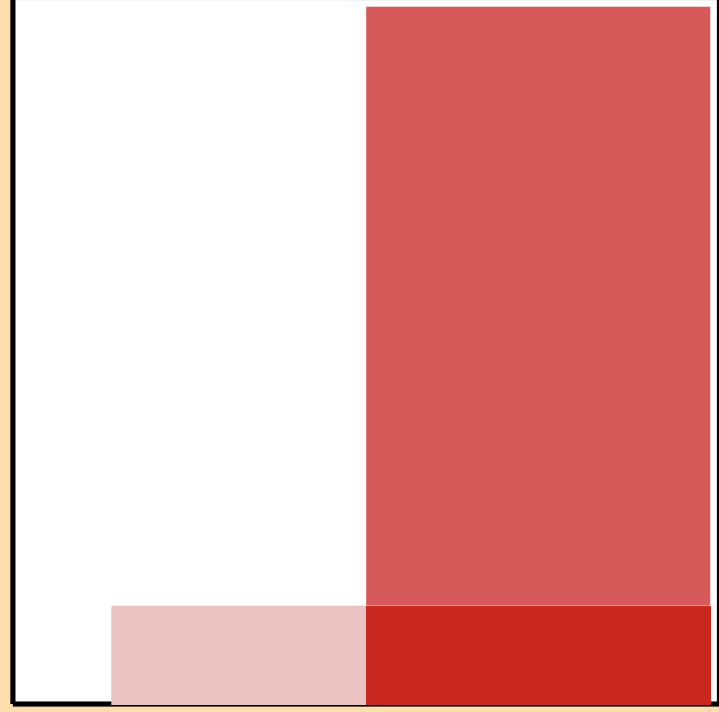
\Delta\sigma/\sigma vs. E for ^{129}\text{Cs}(n,2n)
