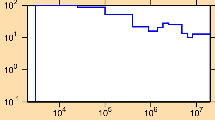
\Delta\sigma/\sigma vs. E for ^{129}\text{Cs}(n,\text{el.})
