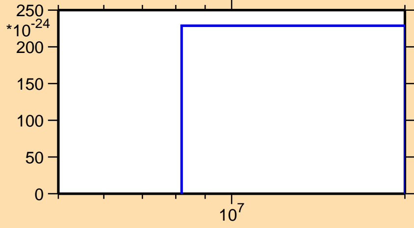
\sigma vs. E for ^{129}\text{Cs} (mt 11)
