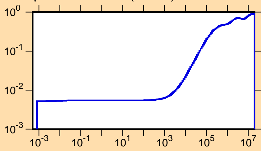
\mu vs. E for ^{130}\text{Cs}(\text{mt251})
