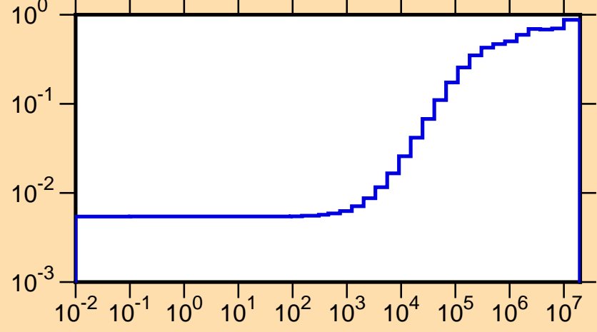
\mu vs. E for ^{130}\text{Cs}(\text{mt251})
