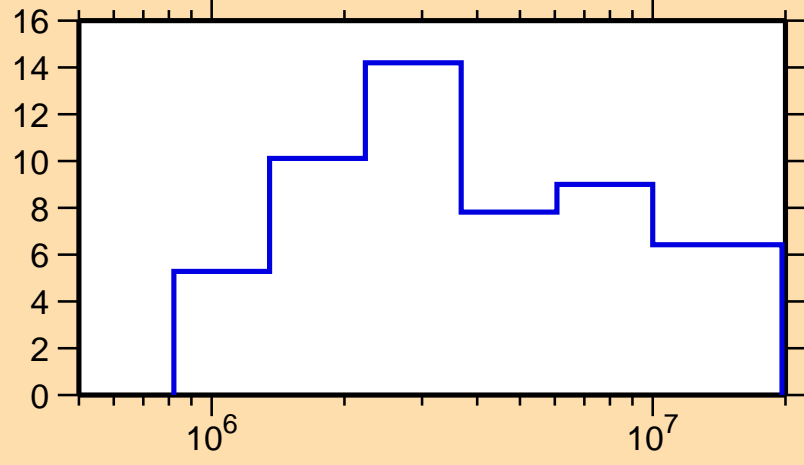
\Delta\sigma/\sigma vs. E for ^{130}\text{Cs}(n, el.)
