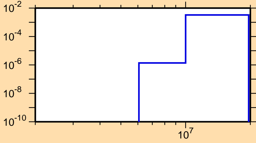
\sigma vs. E for ^{130}\text{Cs}(n,d)
