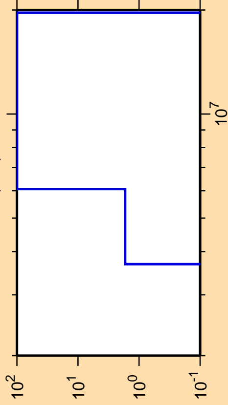
\Delta\sigma/\sigma vs. E for ^{130}\text{Cs}(n,d)
