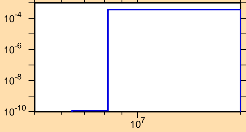
\sigma vs. E for ^{130}\text{Cs}(n,n\alpha)
