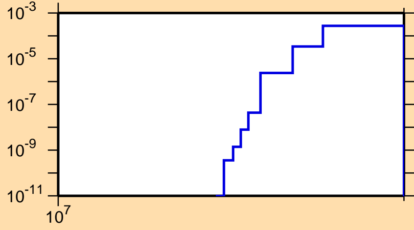
\sigma vs. E for ^{130}\text{Cs}(n,2np)
