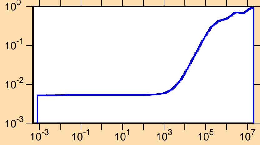
\mu vs. E for ^{131}\text{Cs}(\text{mt251})
