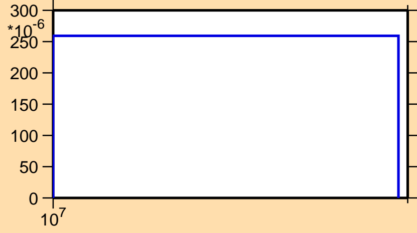
\sigma vs. E for ^{131}\text{Cs}(n,3n)
