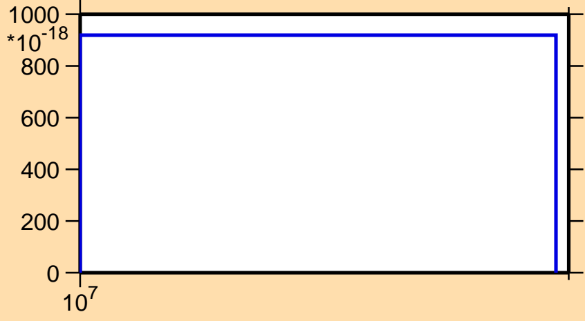
\sigma vs. E for ^{131}\text{Cs} (mt 45)
