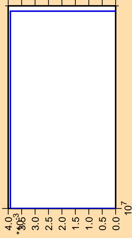
\Delta\sigma/\sigma vs. E for ^{131}\text{Cs} (mt 45)
