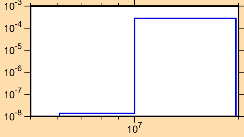
\sigma vs. E for ^{131}\text{Cs}(n,n\alpha)
