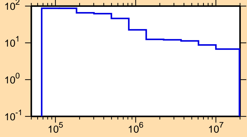
\Delta\sigma/\sigma vs. E for ^{131}\text{Cs}(n,\text{nonel.})
