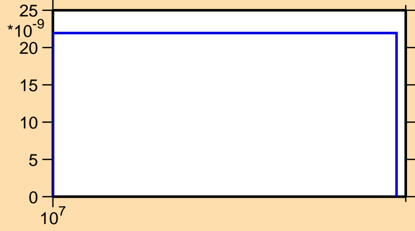
\sigma vs. E for ^{131}\text{Cs}(n,2np)
