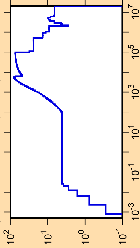
\Delta\mu/\mu vs. E for ^{133}\text{Cs}(\text{mt251})
