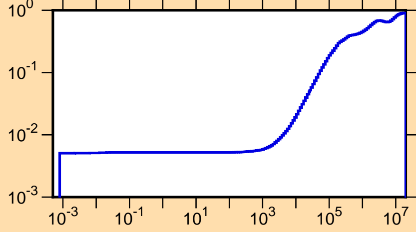
\mu vs. E for ^{133}\text{Cs}(\text{mt251})
