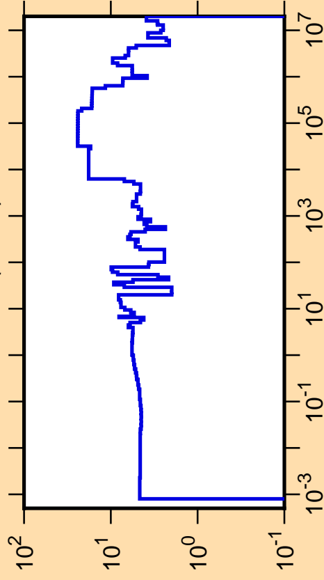
\Delta\sigma/\sigma vs. E for ^{133}\text{Cs}(n,\text{tot.})
