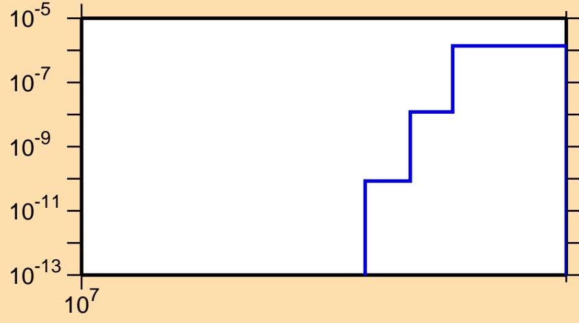
\sigma vs. E for ^{133}\text{Cs}(n,\text{nd})
