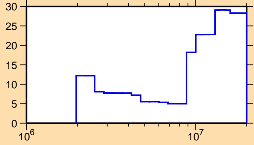
\Delta\sigma/\sigma vs. E for ^{133}\text{Cs}(n,inel.)
