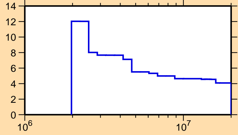
\Delta\sigma/\sigma vs. E for ^{133}\text{Cs}(n,n\text{onel.})
