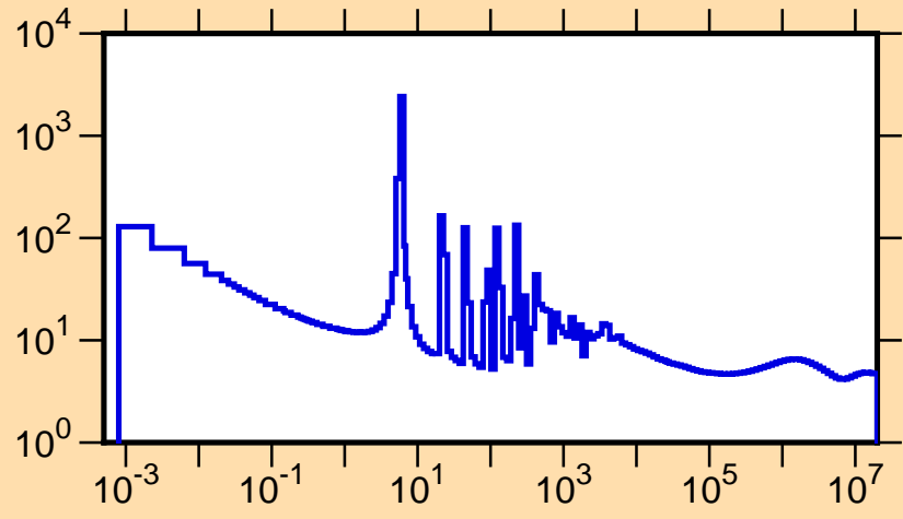
\sigma vs. E for ^{133}\text{Cs}(n,\text{tot.})
