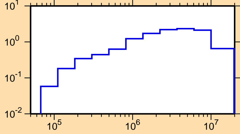
\sigma vs. E for ^{133}\text{Cs}(n,\text{inel.})
