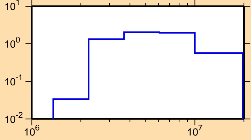
\sigma vs. E for ^{133}\text{Cs}(n,n\text{cont.})
