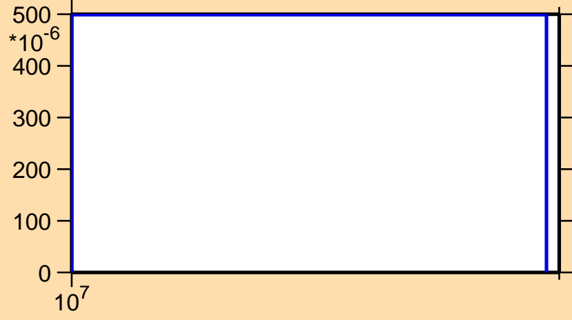
\sigma vs. E for ^{133}\text{Cs}(n,3n)
