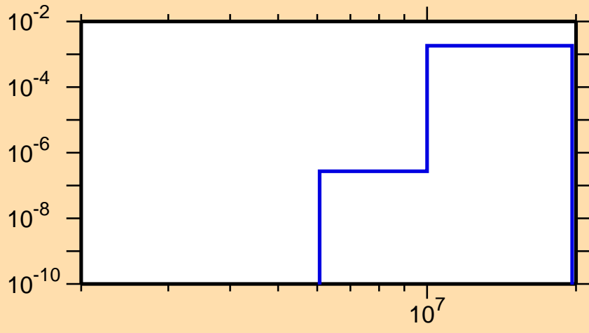
\sigma vs. E for ^{133}\text{Cs}(n,d)
