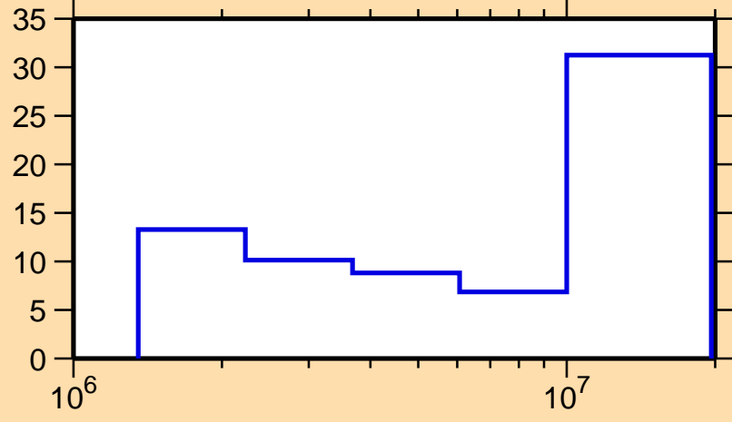
\Delta\sigma/\sigma vs. E for ^{133}\text{Cs}(n,n\text{cont.})
