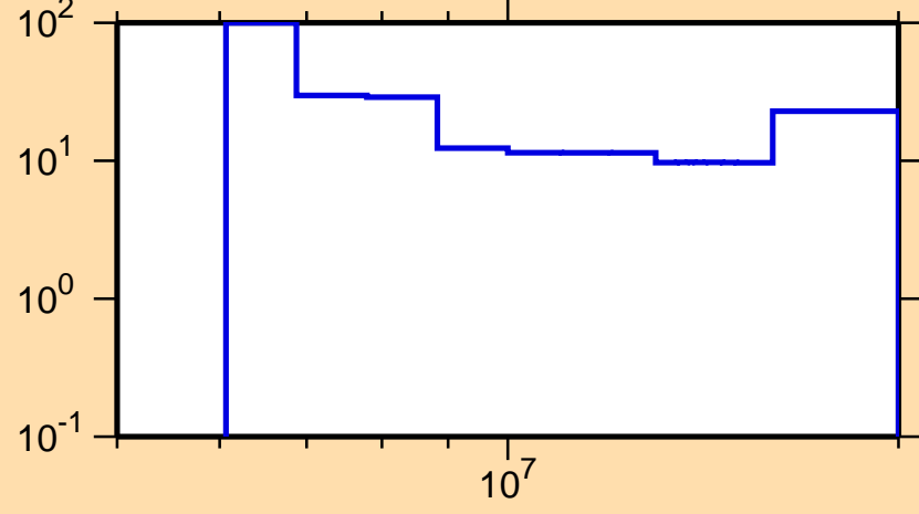
\Delta\sigma/\sigma vs. E for ^{134}\text{Cs}(n,2n)
