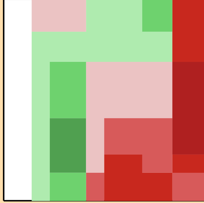
\Delta\sigma/\sigma vs. E for ^{134}\text{Cs}(n,2n)
