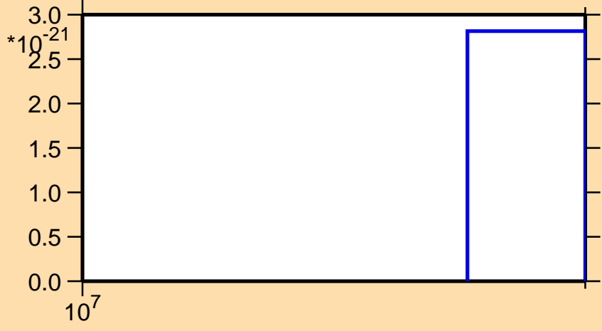
\sigma vs. E for ^{134}\text{Cs} (mt 11)
