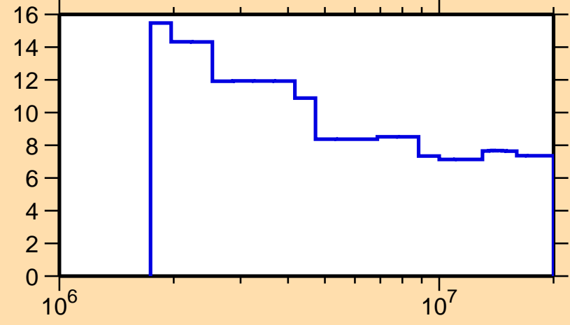
\Delta\sigma/\sigma vs. E for ^{135}\text{Cs}(n,n\text{onel.})
