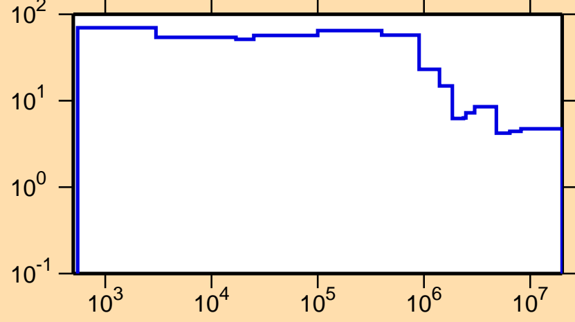
\Delta\sigma/\sigma vs. E for ^{135}\text{Cs}(n,\text{nonel.})
