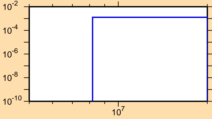
\sigma vs. E for ^{136}\text{Cs}(n,d)
