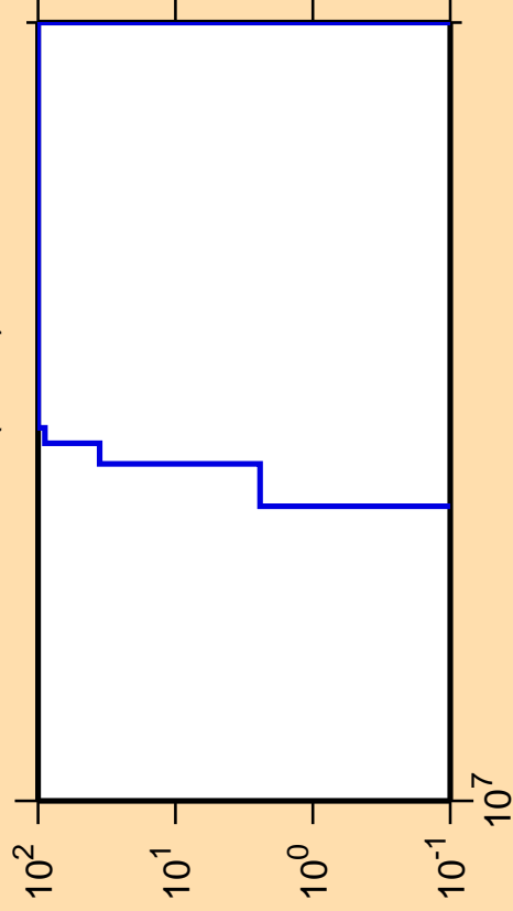
\Delta\sigma/\sigma vs. E for ^{136}\text{Cs}(n,nd)
