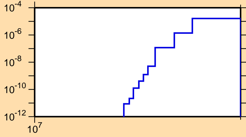
\sigma vs. E for ^{136}\text{Cs}(n,nd)
