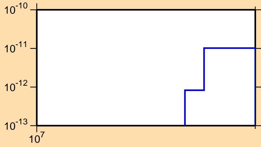
\sigma vs. E for ^{136}\text{Cs}(n,p\alpha)
