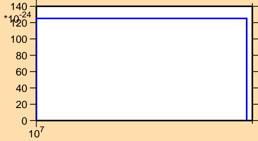
\sigma vs. E for ^{136}\text{Cs} (mt 11)
