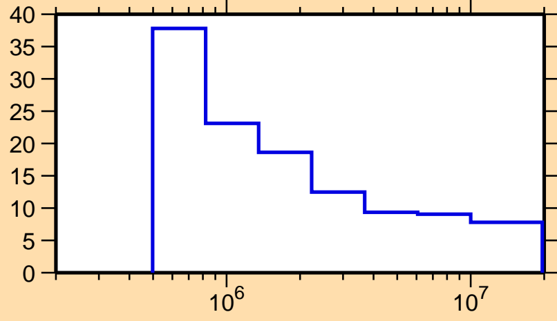
\Delta\sigma/\sigma vs. E for ^{136}\text{Cs}(n,n\text{onel.})
