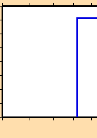
\sigma vs. E for ^{136}\text{Cs}(n,3n)
