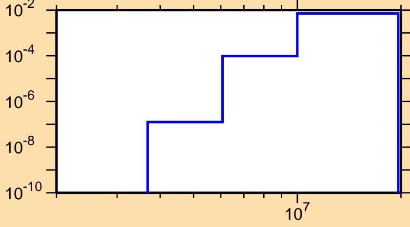
\sigma vs. E for ^{138}\text{Cs}(n,p)
