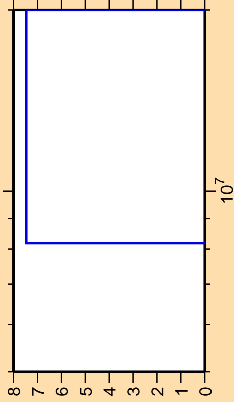
\Delta\sigma/\sigma vs. E for ^{138}\text{Cs}(n,p\alpha)
