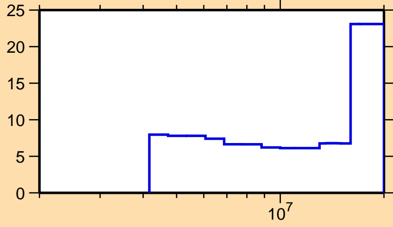
\Delta\sigma/\sigma vs. E for ^{138}\text{Cs}(n,2n)
