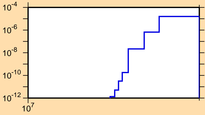
\sigma vs. E for ^{138}\text{Cs}(n,nt)
