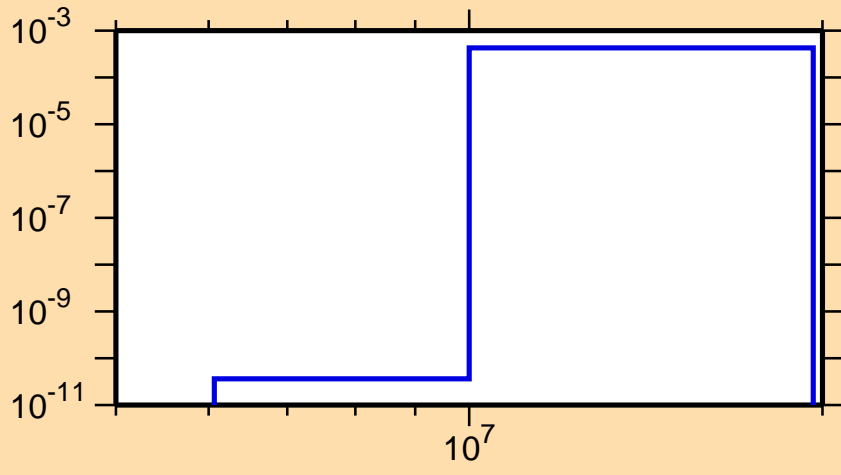
\sigma vs. E for ^{138}\text{Cs}(n,d)
