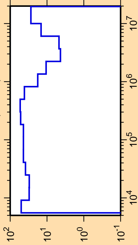
\Delta\sigma/\sigma vs. E for ^{138}\text{Cs}(n,\text{inel.})
