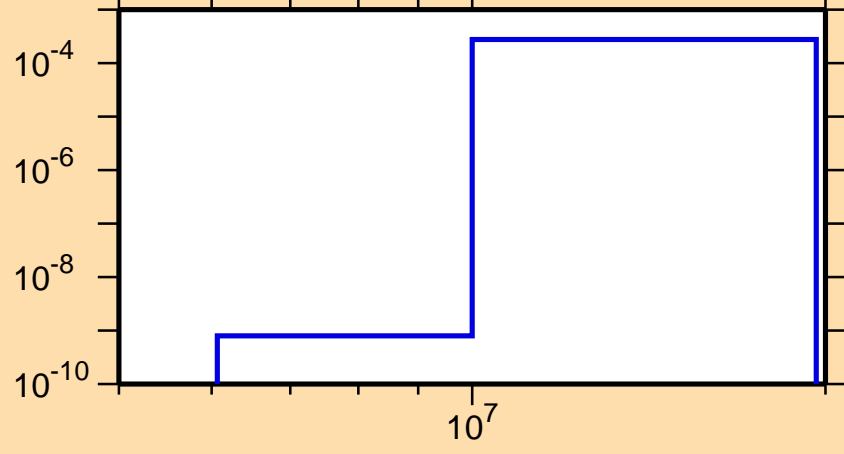
\sigma vs. E for ^{138}\text{Cs}(n,n\alpha)
