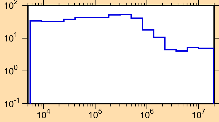
\Delta\sigma/\sigma vs. E for ^{138}\text{Cs}(n,\text{nonel.})
