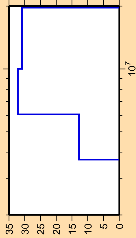
\Delta\sigma/\sigma vs. E for ^{138}\text{Cs}(n,p)
