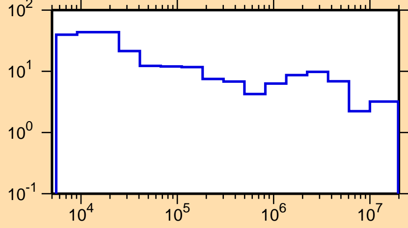
\Delta\sigma/\sigma vs. E for ^{138}\text{Cs}(n,\text{el.})
