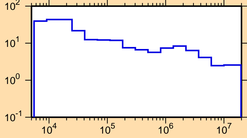
\Delta\sigma/\sigma vs. E for ^{138}\text{Cs}(n,\text{tot.})
