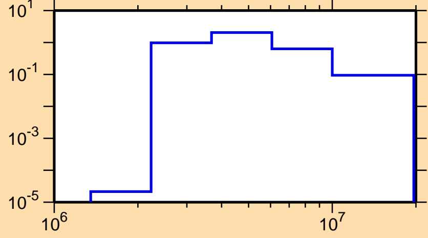
\sigma vs. E for ^{138}\text{Cs}(n,n\text{cont.})
