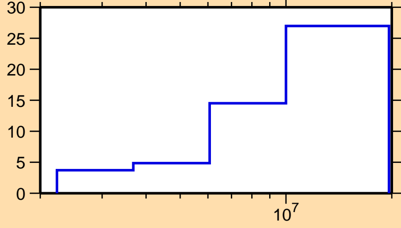
\Delta\sigma/\sigma vs. E for ^{138}\text{Cs}(n,ncont.)
